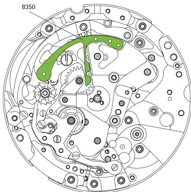
Hammer spring (8350)
