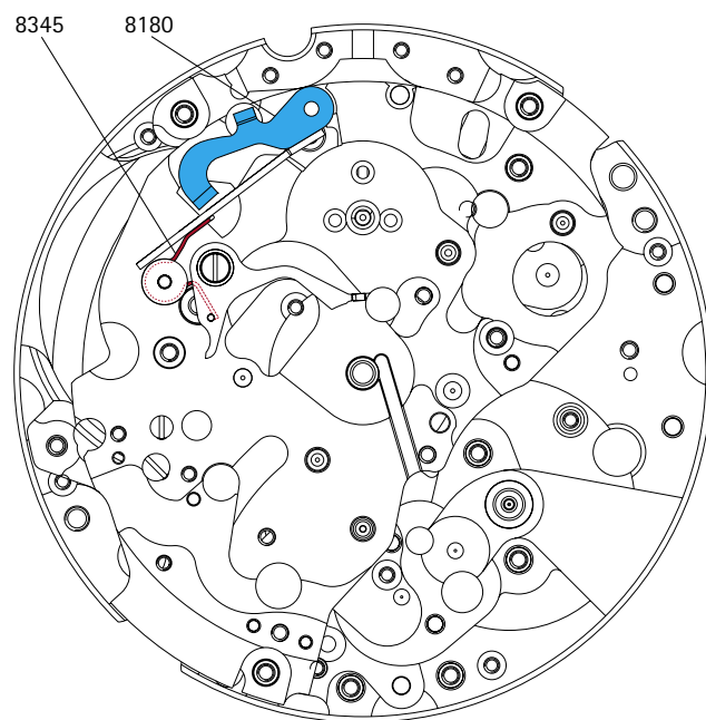
Blocking lever spring (8345) Flyback lever (8180)
